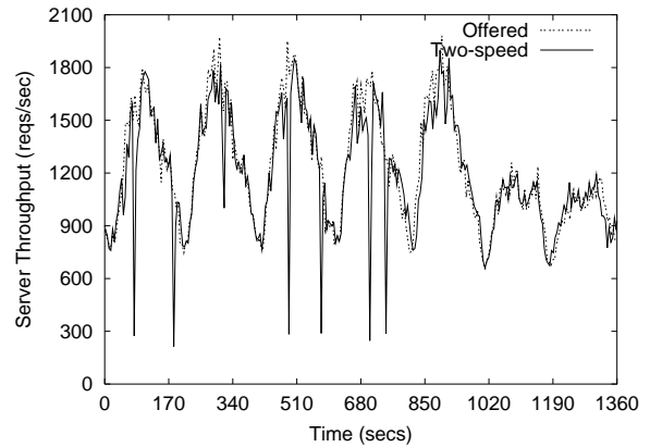
Figure 10: Server throughput for the Clarknet trace with the two-speed disk. Peaks of 80% utilization.
