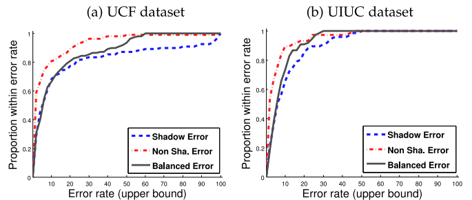
Fig. 6. Per image error distribution within test sets. Proportion of images (Y axis) within a given error rate upper bound threshold (X axis).
