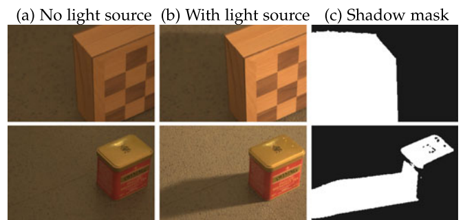
Fig. 4. Generation of 'ground truth' shadow masks on UIUC dataset. Two images of the same scene are taken, with and without blocking a light source. The shadow mask is obtained by considering the difference between two images. This process typically yields a good shadow mask, but not always. Top: Good shadow mask. Bottom: Bad shadow mask; the top of the tea box is not in shadow, and should have not been a part of the shadow mask.
