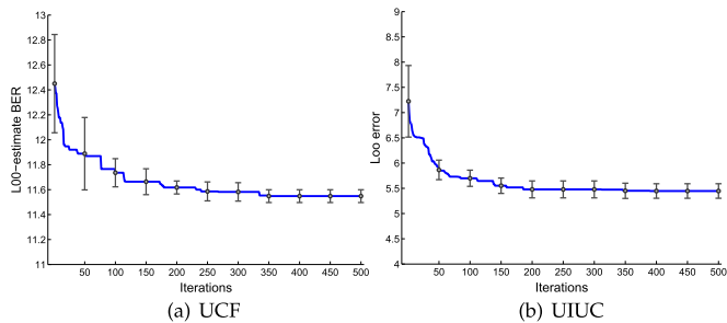
Fig. 7. Leave-one-out balanced error rate as a function of iterations of the kernel optimization. The optimization algorithm converges after around 300 iterations.
