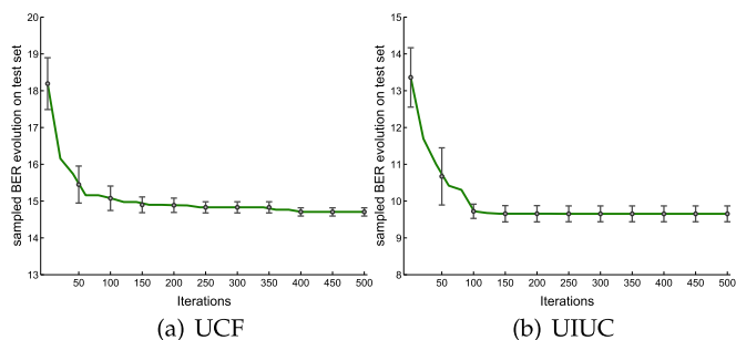
Fig. 8. Balanced error rate on test set. This shows mean BER on the test set over 5 trials. Error bars illustrate variance among trial runs.
