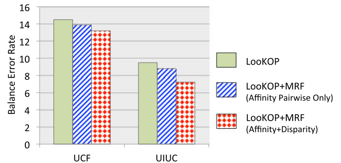
Fig. 5. Benefit of pairwise potentials. This figure shows the balanced error rates for three methods: LookKOP, LookKOP with Affinity pairwise potential, and LookKOP with both Affinity and Disparity pairwise potentials.
