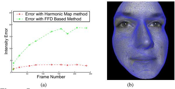
Figure 5. (a) The plot of error between Our method and the FFD Based method (b) FFD breaks down while tracking large deformations. We can see folds and clustering of nodes around the rim of the eyes and lips
