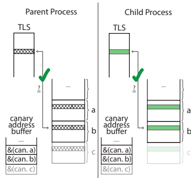
(d) Epilogue checks work as expected since all stack canaries are consistent with the canary in the TLS.
