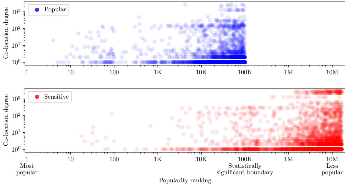
Fig. 11. Co-location degree vs. popularity ranking distribution of successfully fingerprinted websites . “Popular” corresponds to 90,231 fingerprinted websites from the Tranco list’s top-100K most popular domains, while “Sensitive” corresponds to 104,983 fingerprinted websites from 126,597 sensitive domains chosen from Alexa’s sensitive categories that span the whole ranking spectrum. 5,687 fingerprinted websites are common between the two sets.
