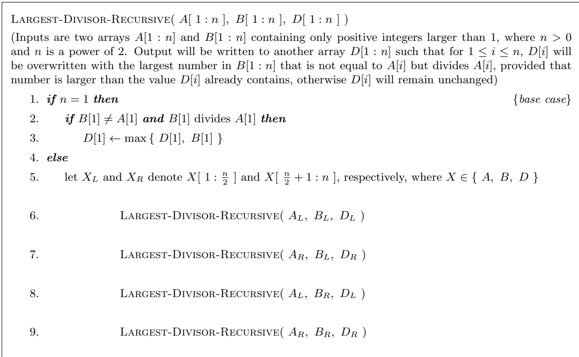
Figure 5: Finds the largest divisor of each entry of A[1 : n] from a given array B[1 : n] . Assumes that each entry of D[1 : n] has already been initialized to 0 before making the initial function call.
