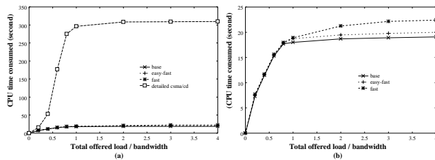
Figure 10. The CPU time consumed for 10 seconds simulations of 10 Mbps Ethernet link with packet size = 512 bytes and buffer size = 8 packets ((b) is the zoomed version of the three curves in the lower portion of (a)).
