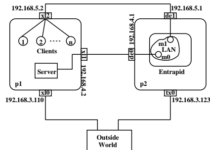
Figure 12. The testbed setting.
