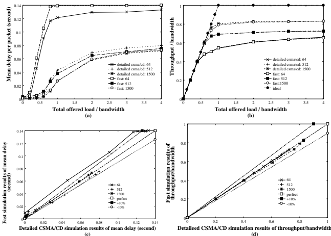
Figure 9. The simulation results for Fast Ethernet Simulation and CSMA/CD simulation for packet size = 64, 512, and 1500 bytes and buffer size = 4500 bytes: (a) delay versus total offered load, (b) throughput versus total offered load, (c) Q-Q plot of (a), (d) Q-Q plot of (b).
