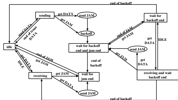
Figure 2. State diagram of distributed CSMA/CD simulation
