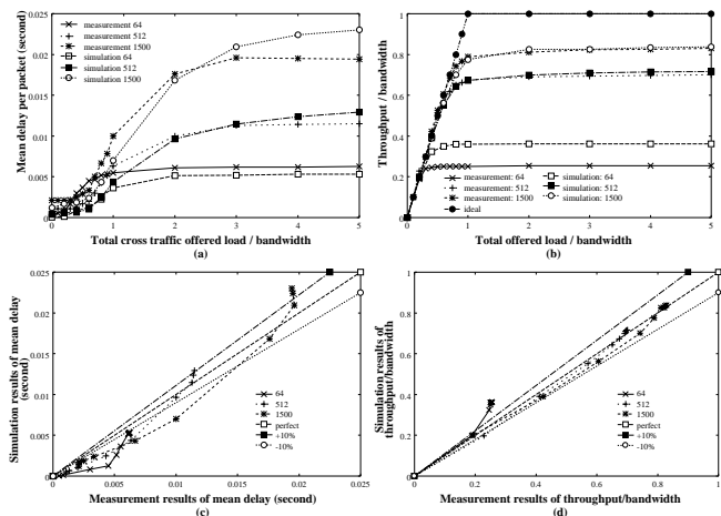
Figure 3. 10 Mbps Ethernet measurement and simulation results (under the same choices of parameters in Gonsalves’ work) on mean packet delay and link throughput. (a) delay versus total cross traffic offered load, (b) throughput versus total offered load, (c) Q-Q plot of (a), (d) Q-Q plot of (b).
