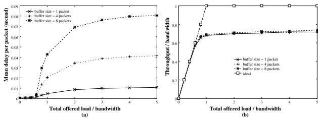
Figure 4. 10 Mbps Ethernet simulation results with buffer size of 1, 4, 8 packets (packet size = 512 bytes): (a) mean delay versus total offered load, (b) throughput versus total offered load.
