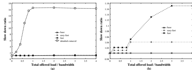
Figure 11. The ratio of CPU time consumed for 10 seconds simulations of 10 Mbps Ethernet link with packet size = 512 bytes and buffer size = 8 packets ((b) is the zoomed version of the three curves in the lower portion of (a)).
