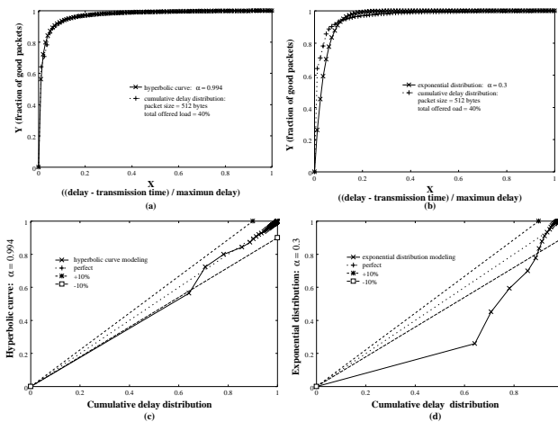
Figure 6. Hyperbolic curves: (a) using hyperbolic curve to model cumulative delay distribution, (b) using exponential distribution to model cumulative delay distribution, (c) Q-Q plot of (a), (d) Q-Q plot of (b).
