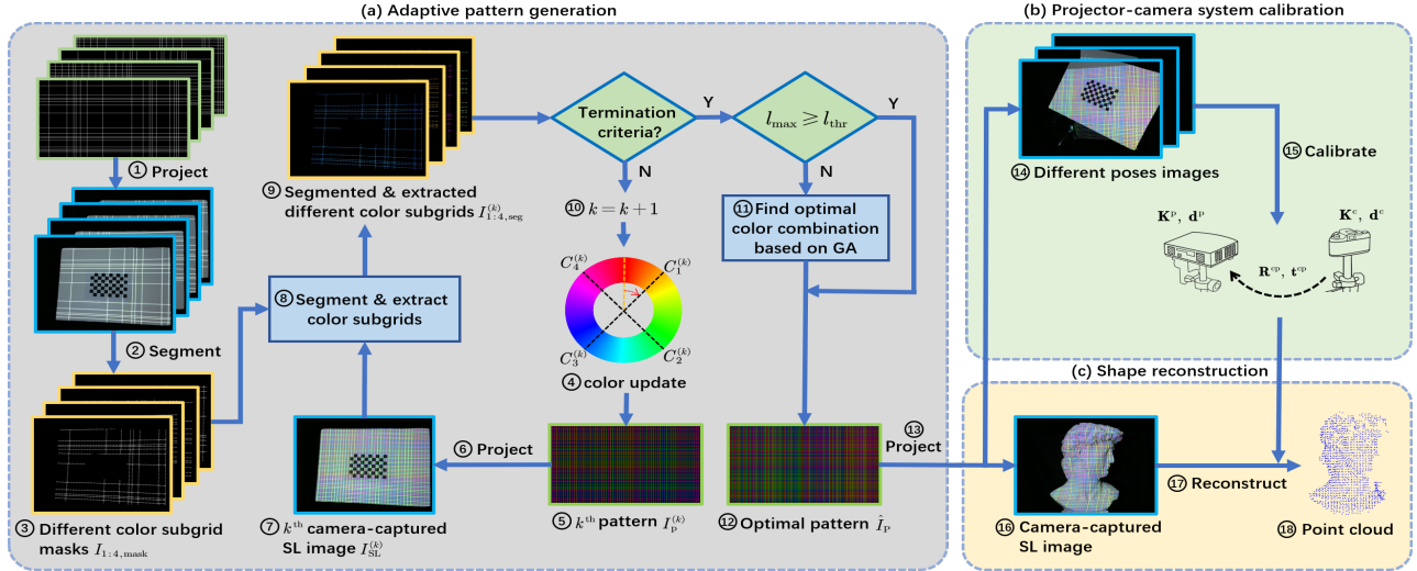
Figure 2: Overview of our adaptive color SL system. Our method can be roughly divided into three parts: (a) adaptive pattern generation, (b) projector-camera system calibration and (c) shape reconstruction. We first project N (e.g., N = 4 ) white subgrid patterns onto the calibration board, and segment them to obtain the corresponding color subgrid masks I_{1:4,mask} for later use. Then, we update the color combination C_{1:4}^{(k)} of our color grid pattern iteratively. In each iteration, we first project the color grid pattern I_p^{(k)} , and capture it as an image I_{SL}^{(k)} . Afterwards, we segment I_{SL}^{(k)} and extract different color subgrids from it using color subgrid masks I_{1:4,mask} . We analyze the segmented and extracted color subgrids I_{1:4,seg}^{(k)} and measure whether we reach the maximum number of iterations or the color distinction score is above the desired threshold l_{thr} (i.e., termination criteria). After the iterative adjustment, if the final color distinction score l_{max} is still lower than the desired optimal score threshold l_{thr} , we use GA to efficiently search for the optimal color combination among all observed colors. Finally, our optimal color grid pattern I_p is generated using the optimal color combination, and used for (b) projector-camera system calibration and (c) shape reconstruction.
