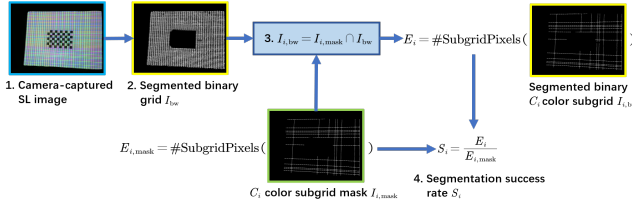
Figure 3: Segmentation success rate calculation. (1) Capture the scene with a color grid pattern as an SL image. (2) Segment the color grid to obtain the binary grid I_{bw} from SL image. (3) Use the C_i color subgrid mask I_{i,mask} to extract the binary C_i color subgrid I_{i,bw} from I_{bw} . (4) Calculate S_i for C_i color using the number of subgrid pixels of the C_i color subgrid mask I_{i,mask} and the C_i color subgrid I_{i,bw} .
