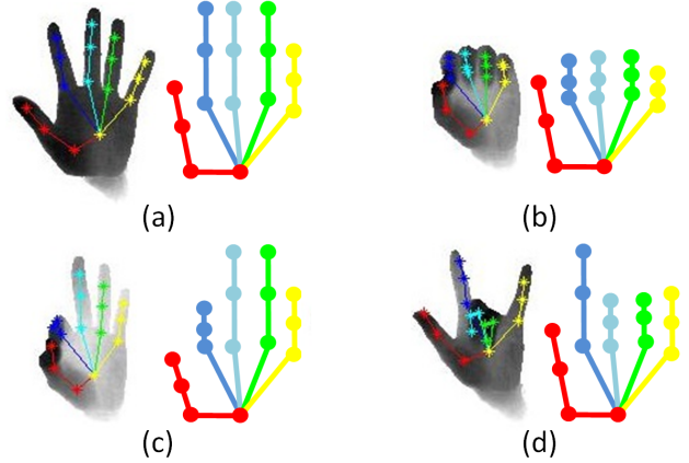
Figure 4. Ideally, all of these four types of hand pose should have same topology structure like (a). However, due to viewpoint and the labeling of raw depth image limitation, (a)(b)(c) and (d) have different hand models. This figure is best viewed in color.
